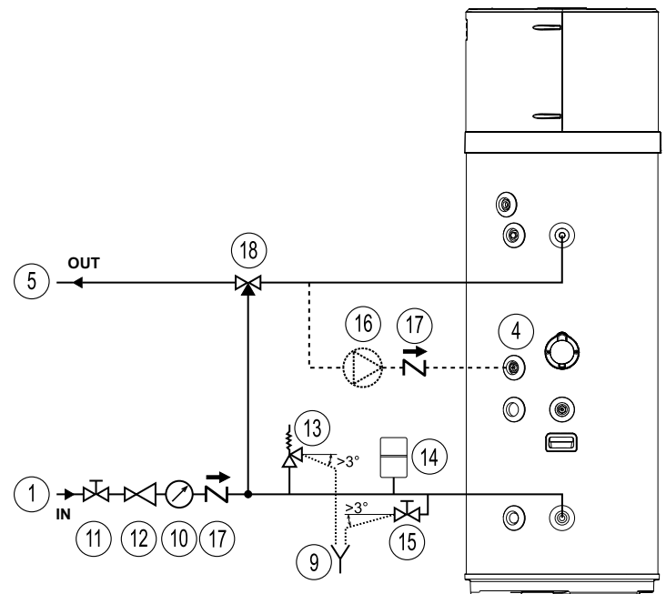
fig. 17- Example of water system
