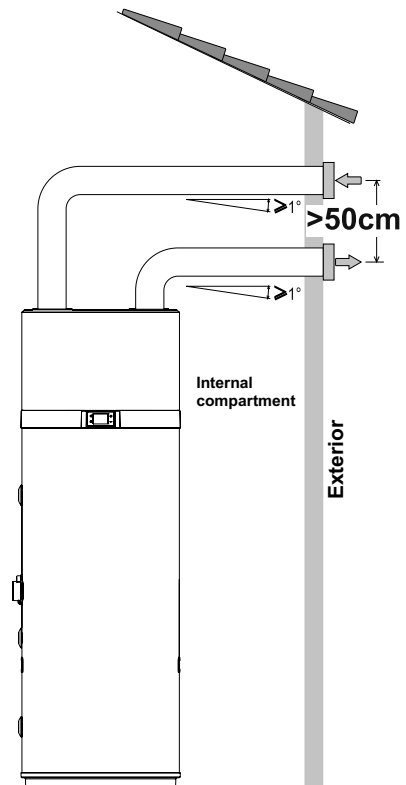
fig. 13- Example of air outlet connection
